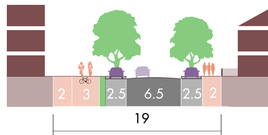
Fig.48 Street sections
