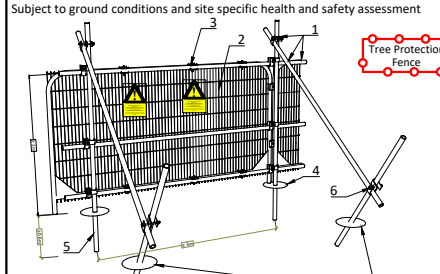
DETAIL 1: Specification For Protective Barrier (Default - BS 5837) Subject to ground conditions and site specific health and safety assessment
